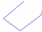
Not a Polygon (open, not closed)
